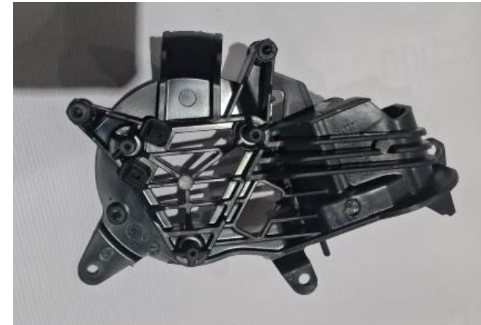
W601 Case Frame Power Fold
