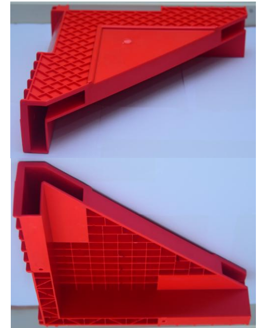
Corner Bracket
