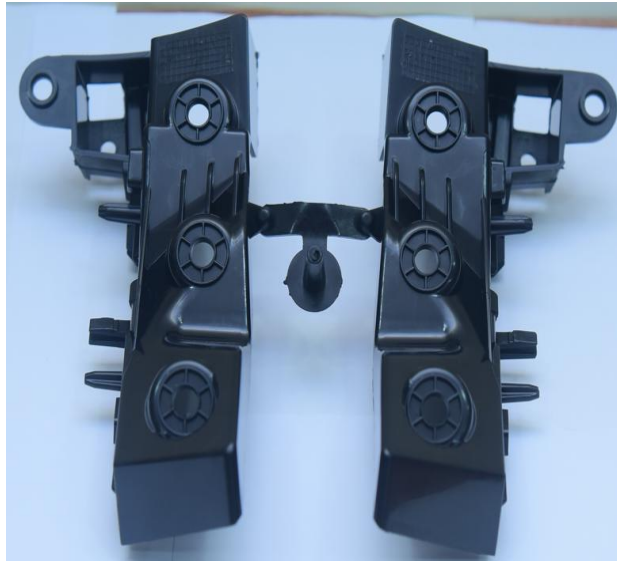
Bumper Bracket
